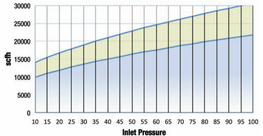
Pressure Drop
