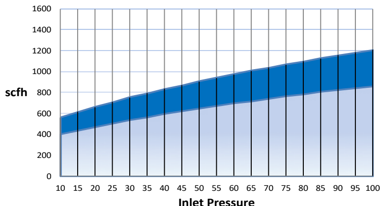
Pressure Drop
