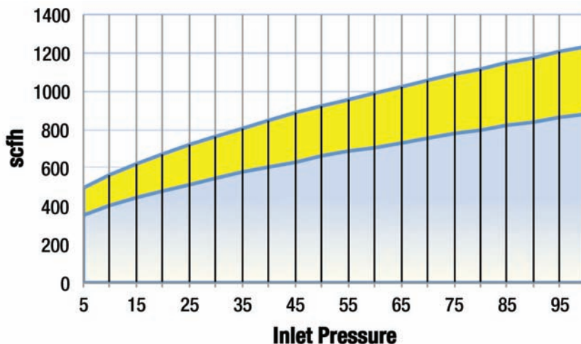
Pressure Drop
