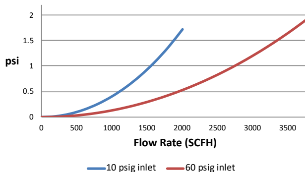
Pressure Drop
