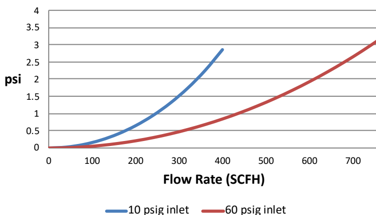
Pressure Drop
