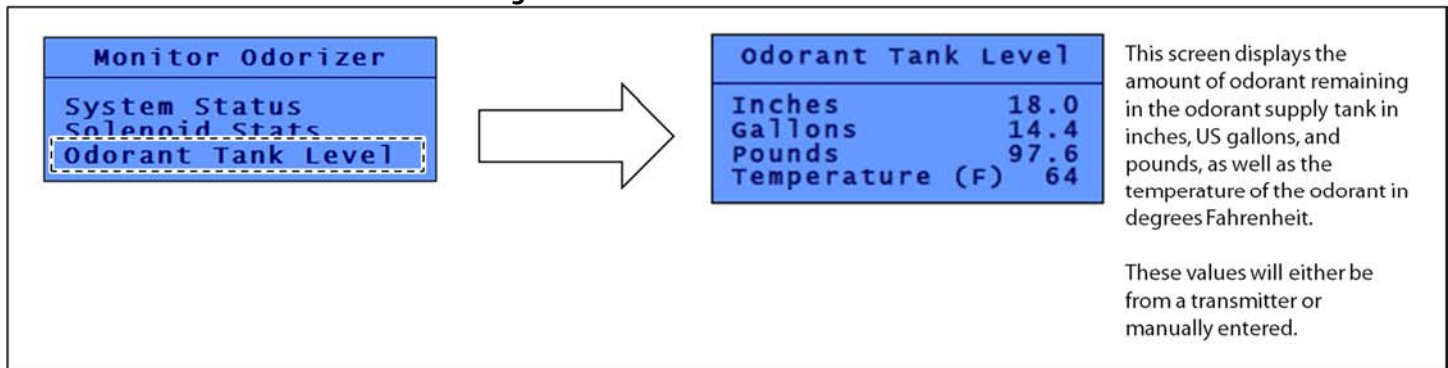
Figure 17: Odorant Tank Level Submenu
