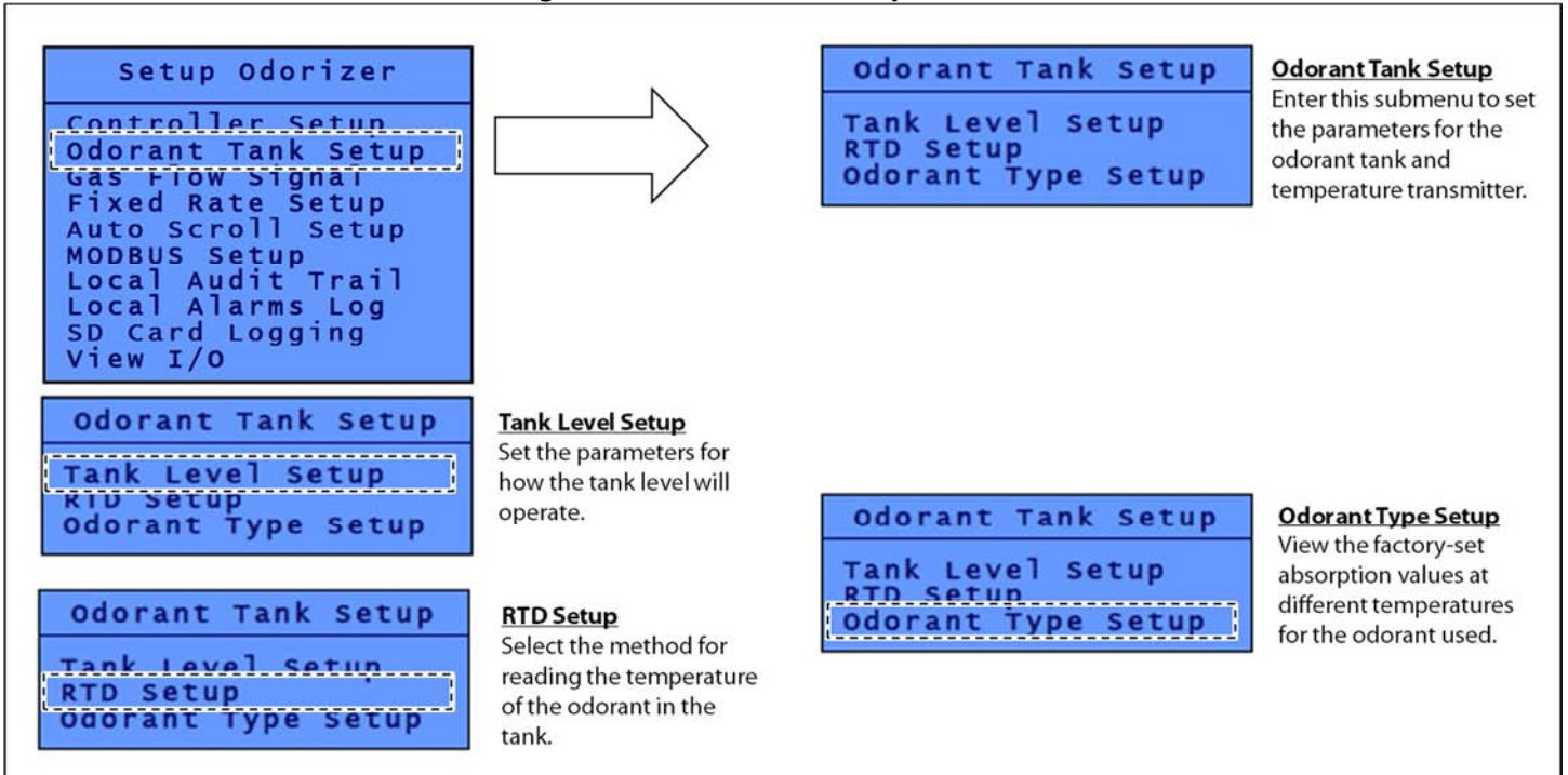
Figure 26: Odorant Tank Setup Submenus
