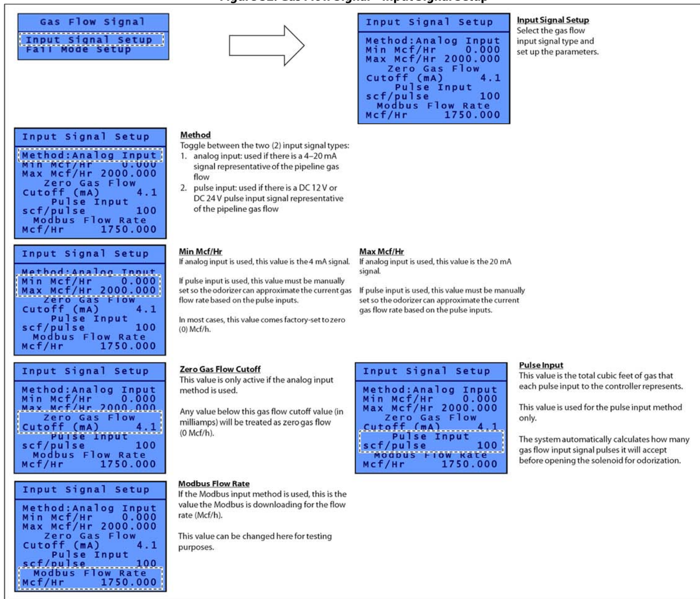
Figure 32: Gas Flow Signal – Input Signal Setup
