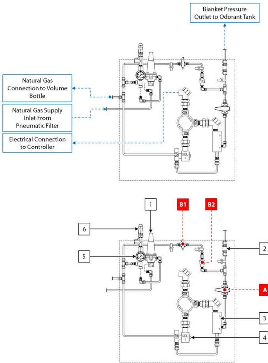
Figure 3: Valve Section – Single Solenoid, \frac{3}{8} " Tubing
