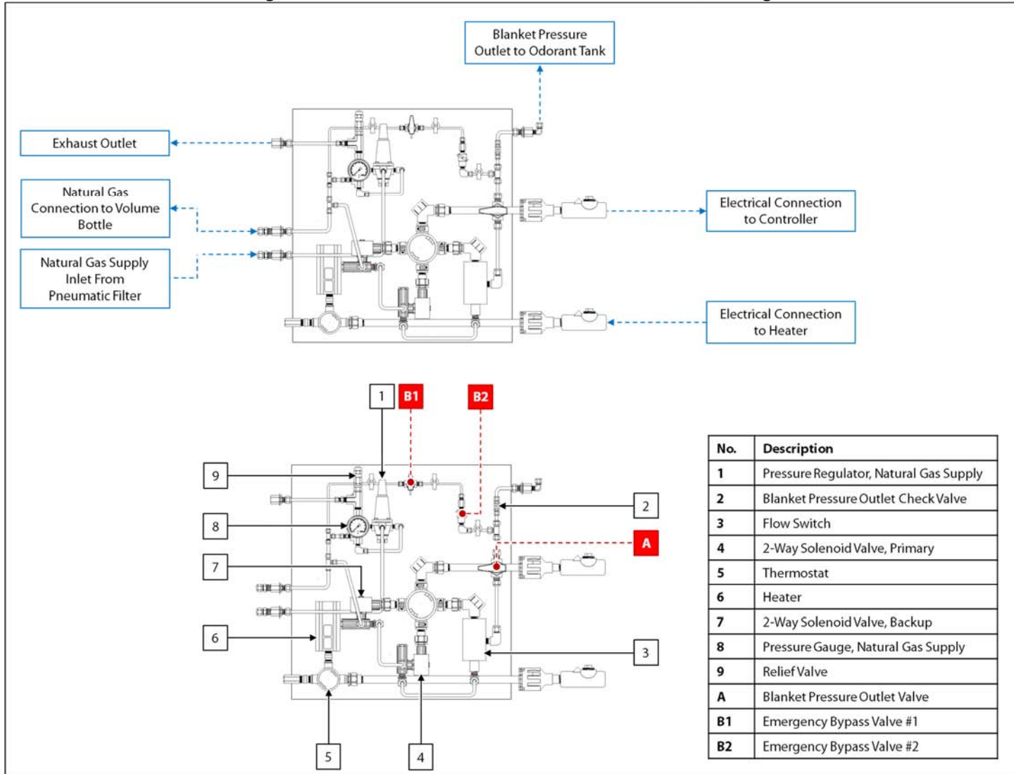
Figure 5: Valve Section – Dual Solenoid With Heater, \frac{3}{8} " Tubing
