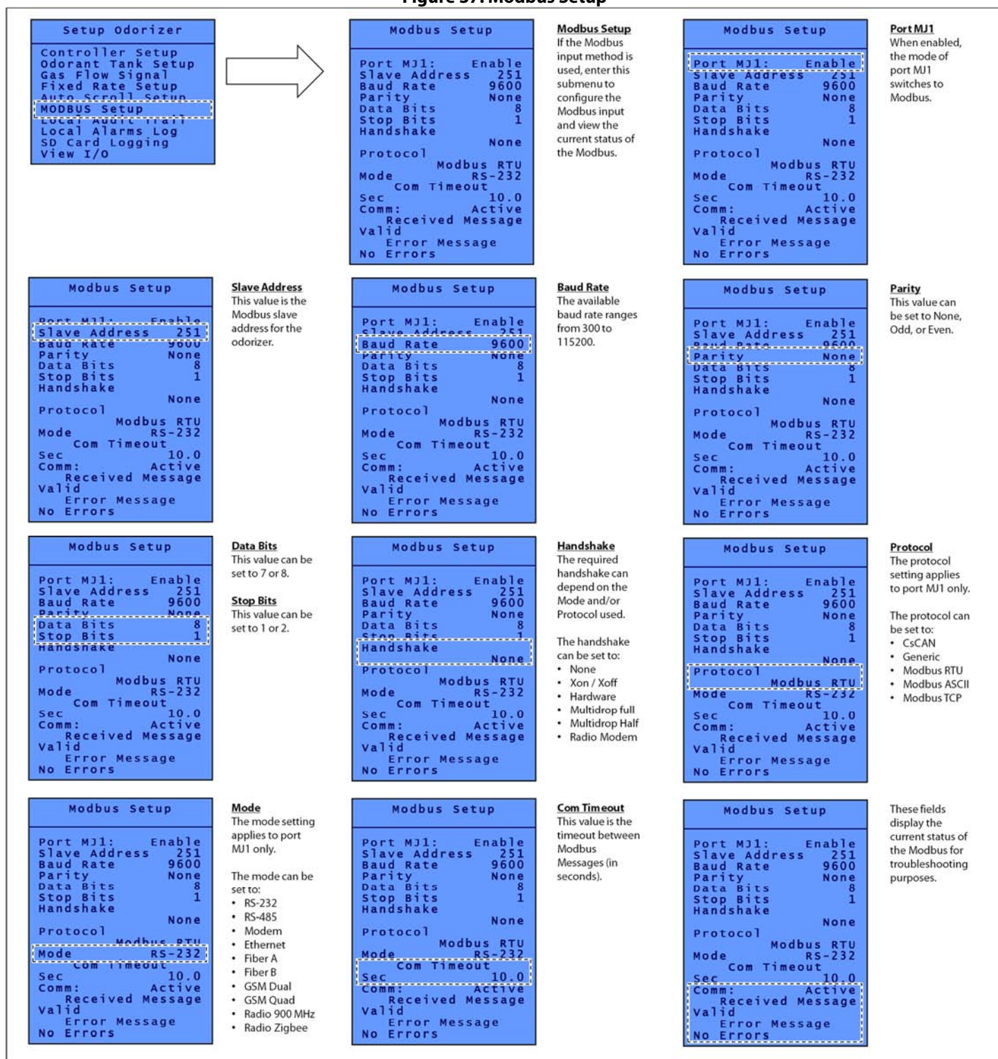
Figure 37: Modbus Setup
