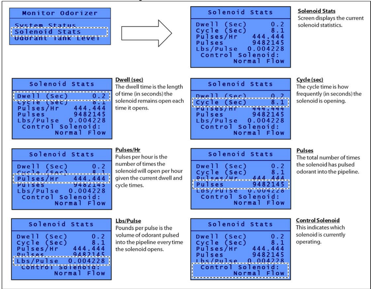
Figure 16: Solenoid Stats Submenu
